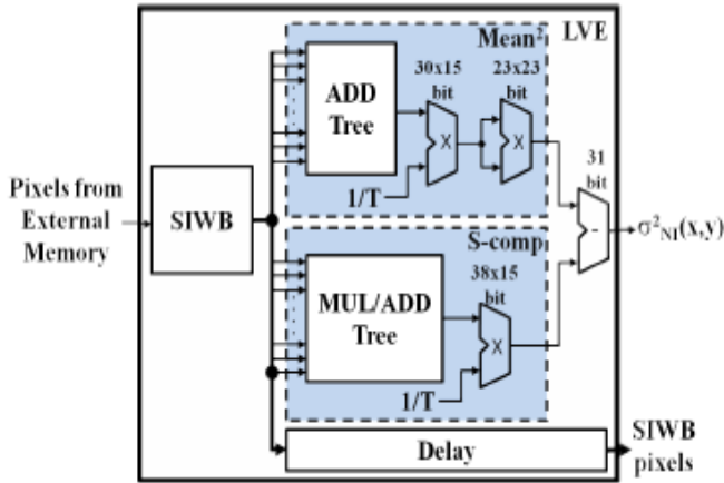
Figure 7: LVE Internal architecture
