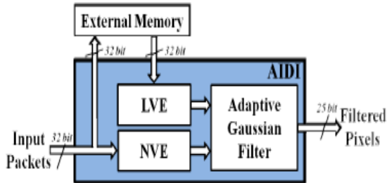
Figure 1: AIDI Internal architecture
