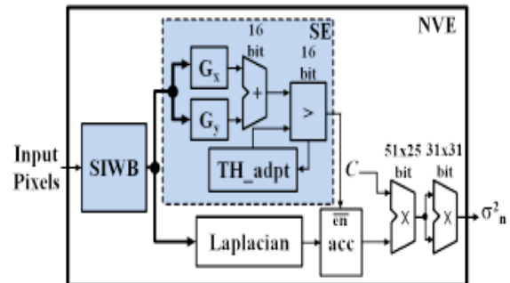
Figure 5: NVE Internal architecture
