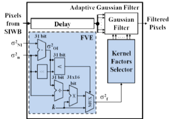
Figure 8: Adaptive Gaussian Internal architecture
