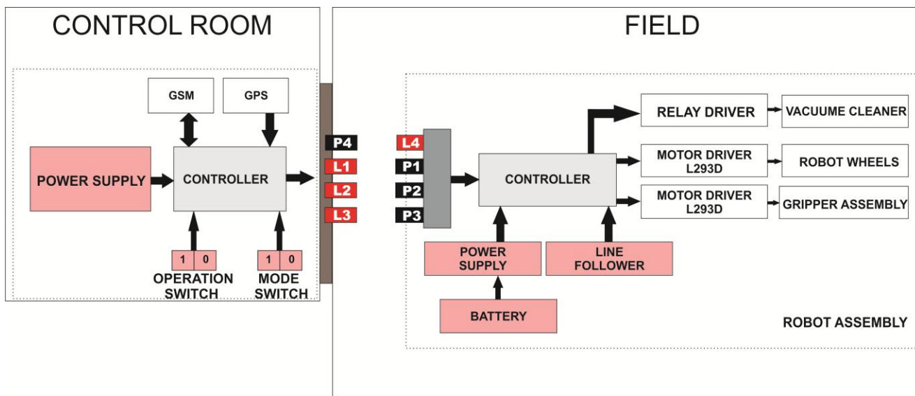
Fig 1 : Block diagram of the overall system
